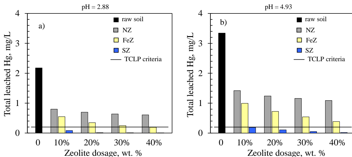
Figure 1. TCLP results of total leached Hg concentration at: a) pH=2.88 and b) pH=4.93.
