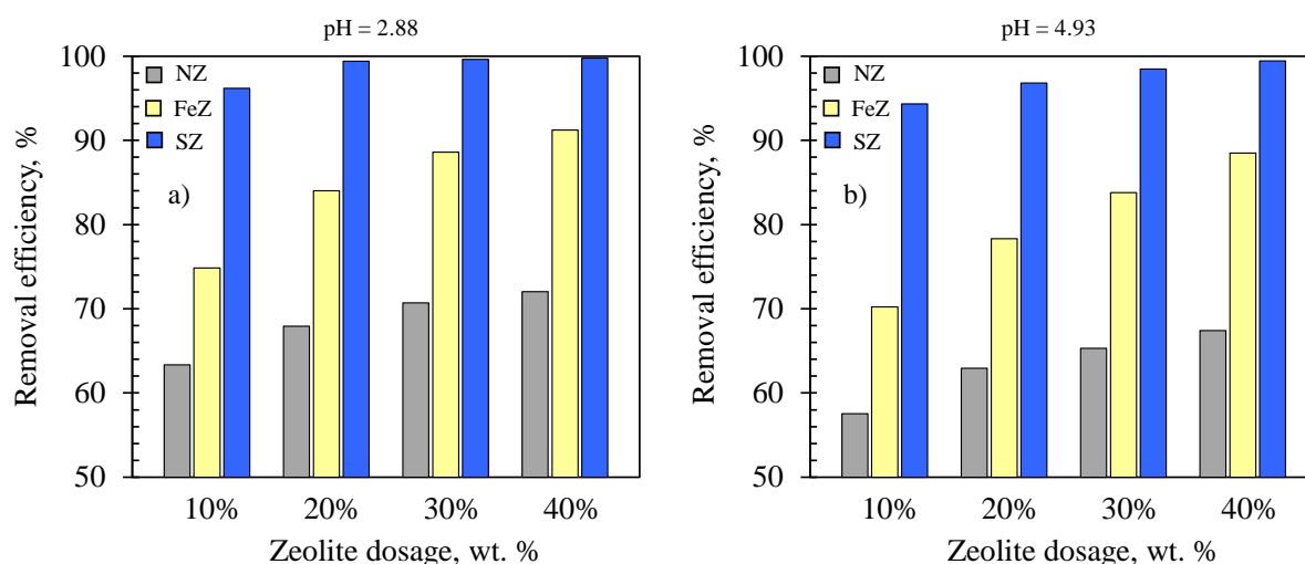
Figure 2. Removal efficiency of leached Hg by addition of different quantities of zeolites at: a) pH=2.88 and b) pH=4.93.
