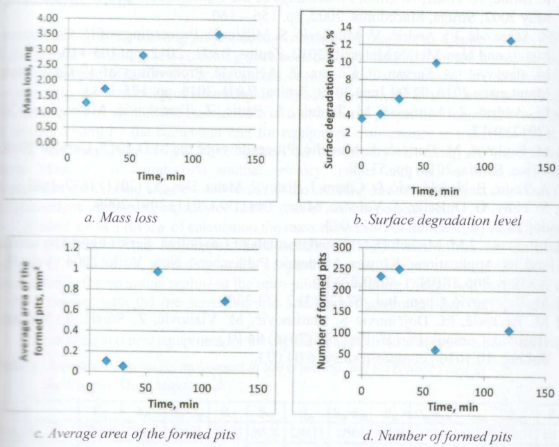
Figure 3 Results of research on development the cavitation damage of basalt samples during the cavitation erosion test
